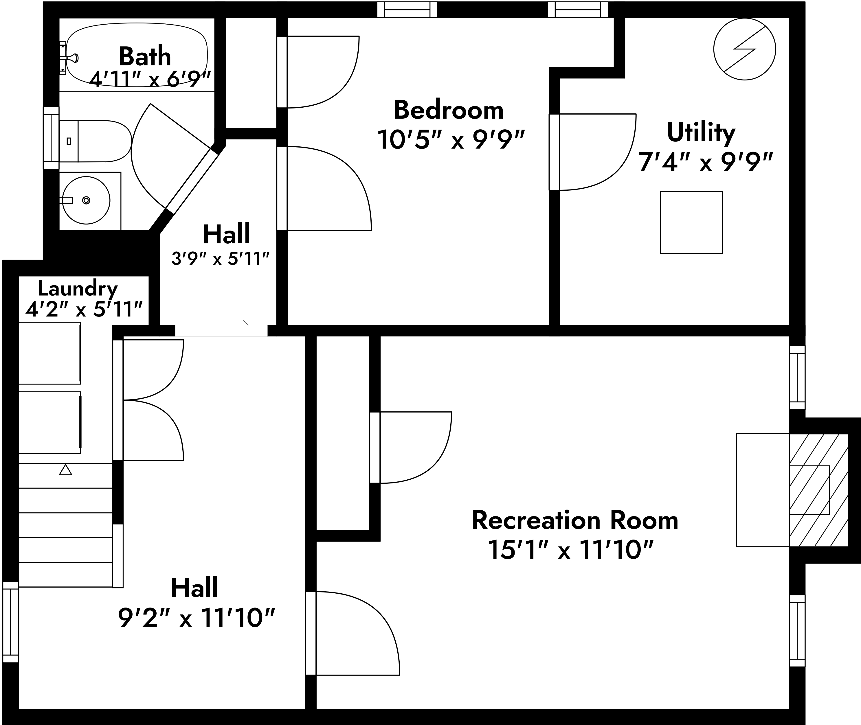
Lower Level
