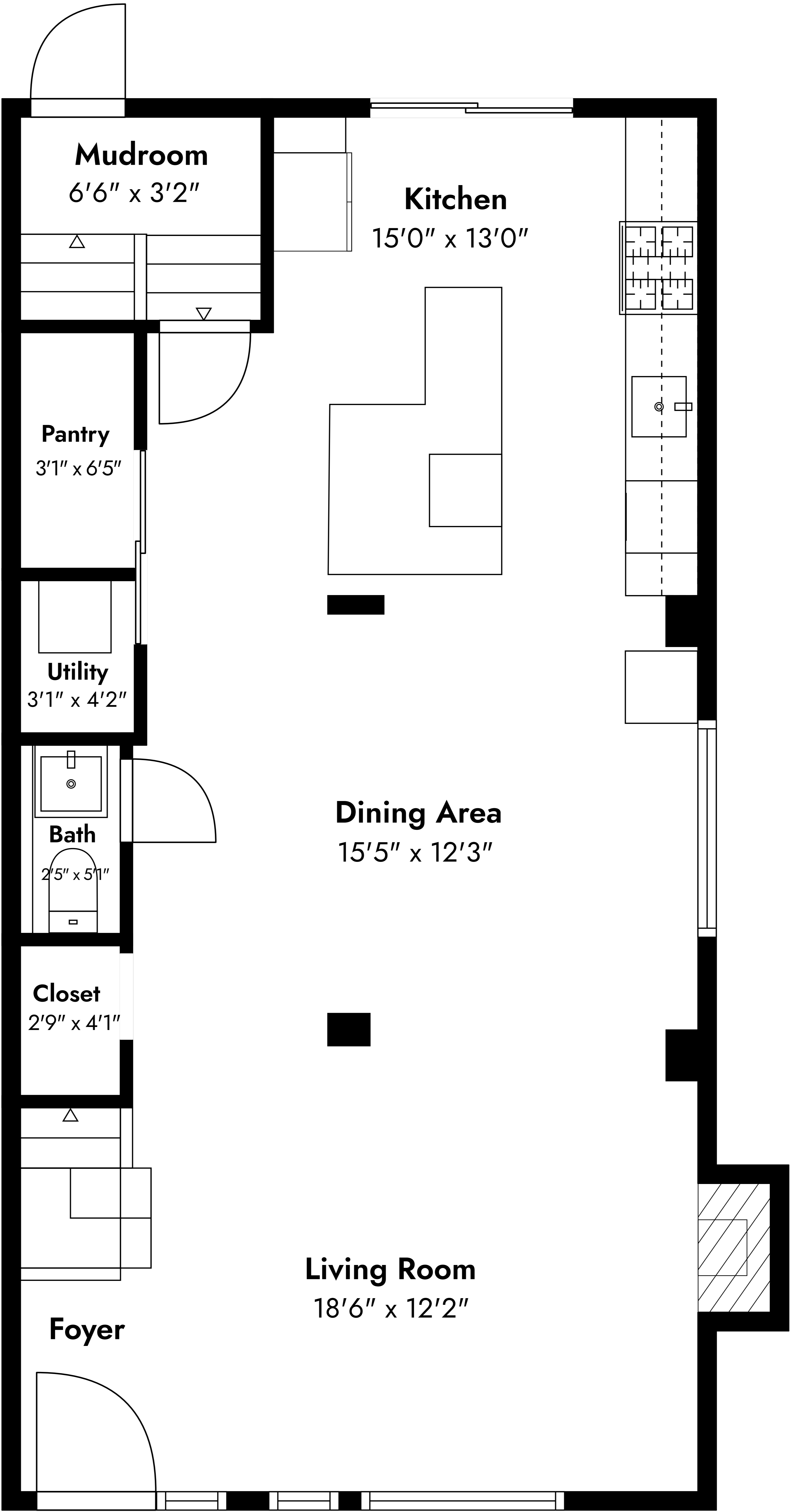
MAIN LEVEL
