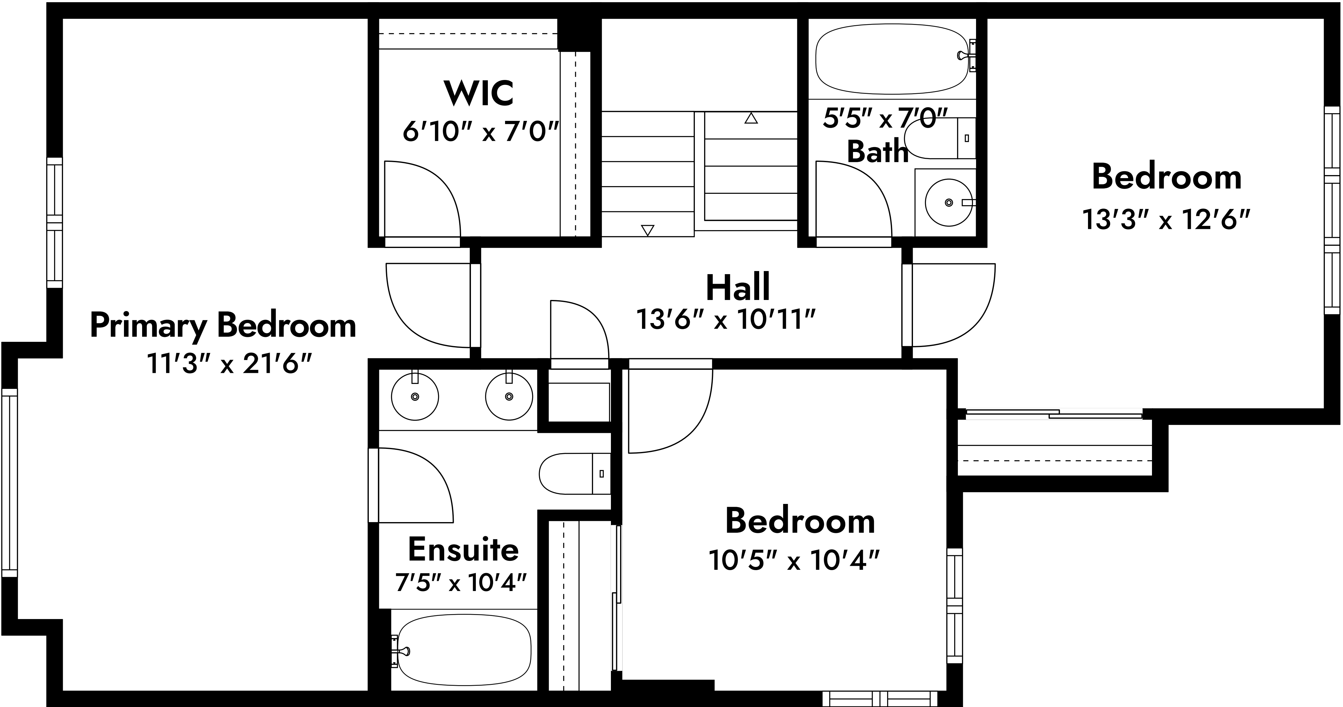
SECOND LEVEL
