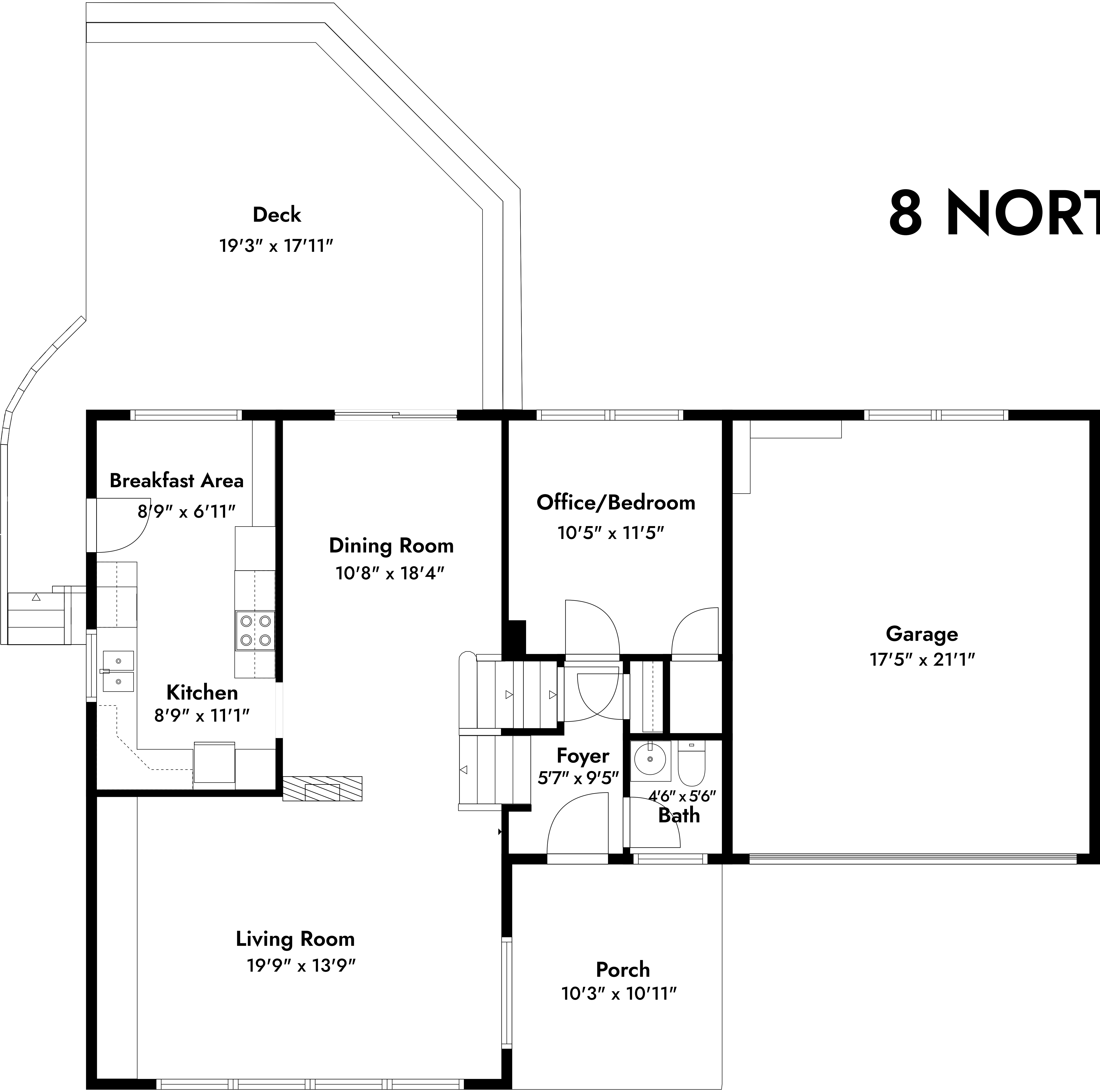
MAIN LEVEL
